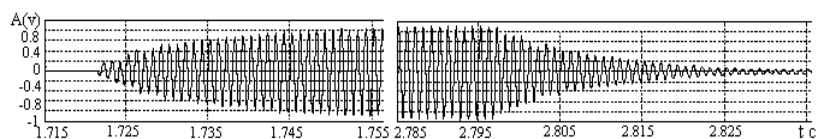
Fig. 4. Reverberation amplitudes at the damping process
