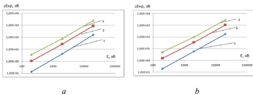
Fig. 1. Ion energy dependence of the additional crystallization energy at different ion charge (curve 1–1, 2–2, 3–3), acting on the D16T aluminum alloy
