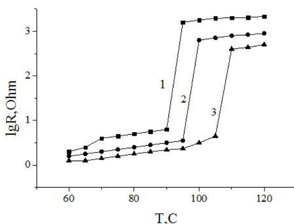
Fig. 2. Dependence of the resistance of the conducting rubbers on the temperature for composites with three contents (Wt%): 1 – PDMVS (40)+P803 (57)+PDC (3); 2 – PDMVS (46)+P357E (10)+P803 (40)+PDC (4); 3 – PDMVS (50)+P803 (30)+P357E (15)+PDC (5)
